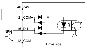
Active-low
