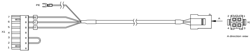
Wiring relation
