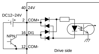
Active-low
