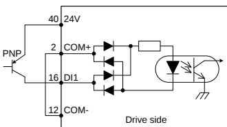
Active-high
