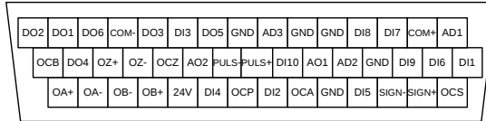
CN1 plug signal layout
