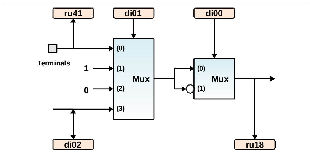
Figure 113: Digital inputs block diagram
