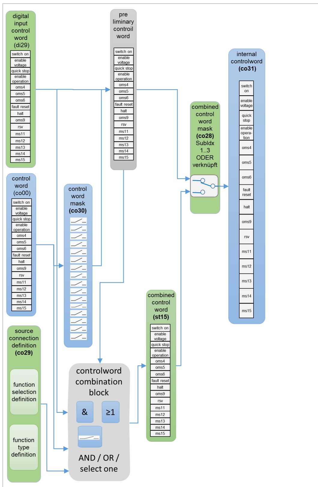
Figure 120: digital input controlword
