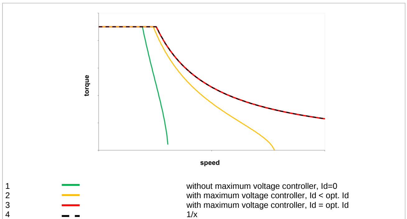
Figure 75: Limit value at synchronous motors
