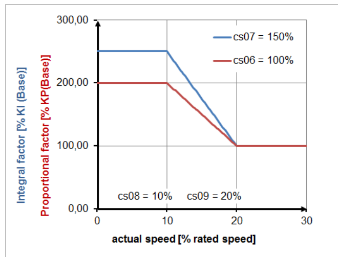
Figure 99: Variable proportional factor (kp) / integral factor (ki) with cs08=10% , cs09=20%
