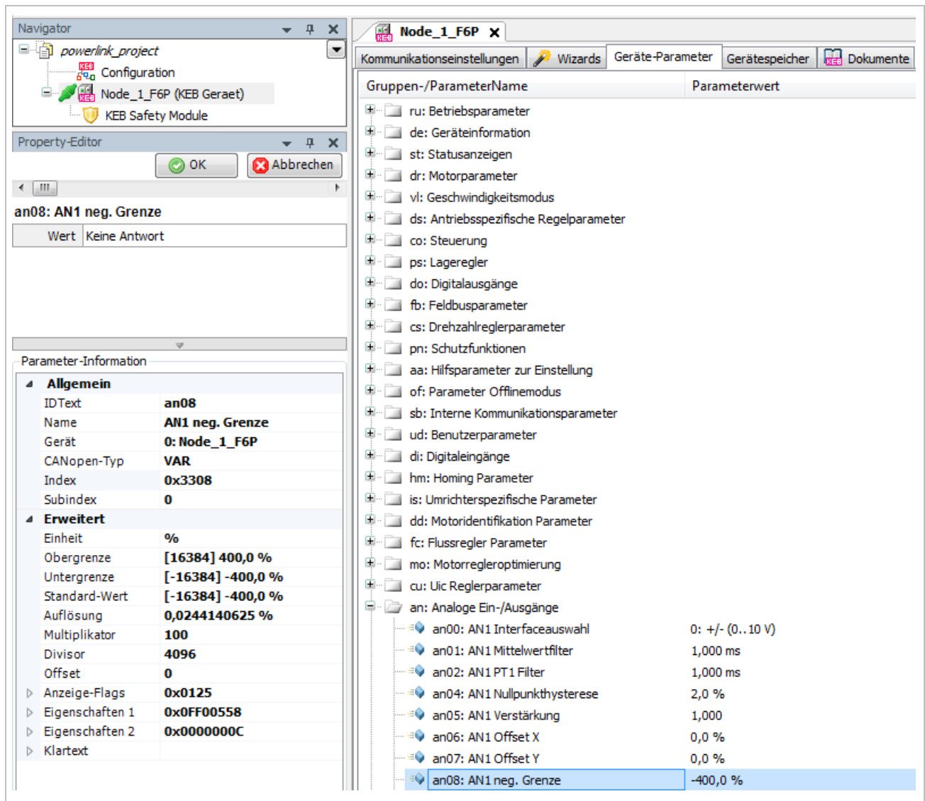
Figure 130: Display object data in COMBIVIS
