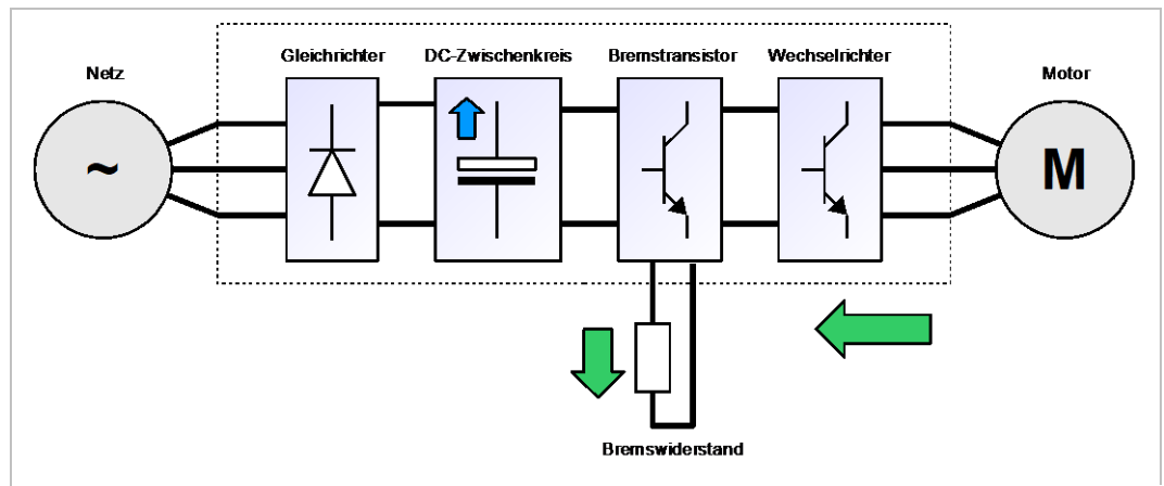
Figure 19: Regenerative operation
