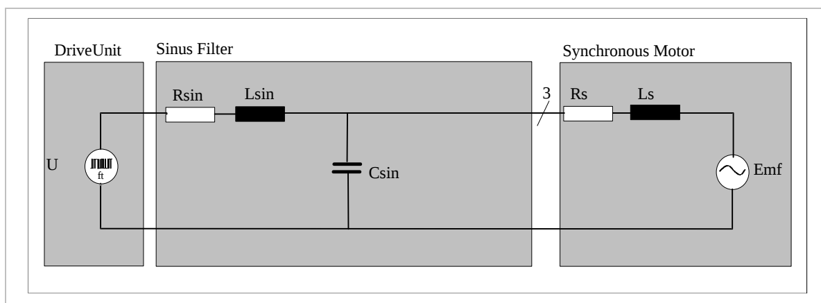
Figure 94: Connection example sinus filter
