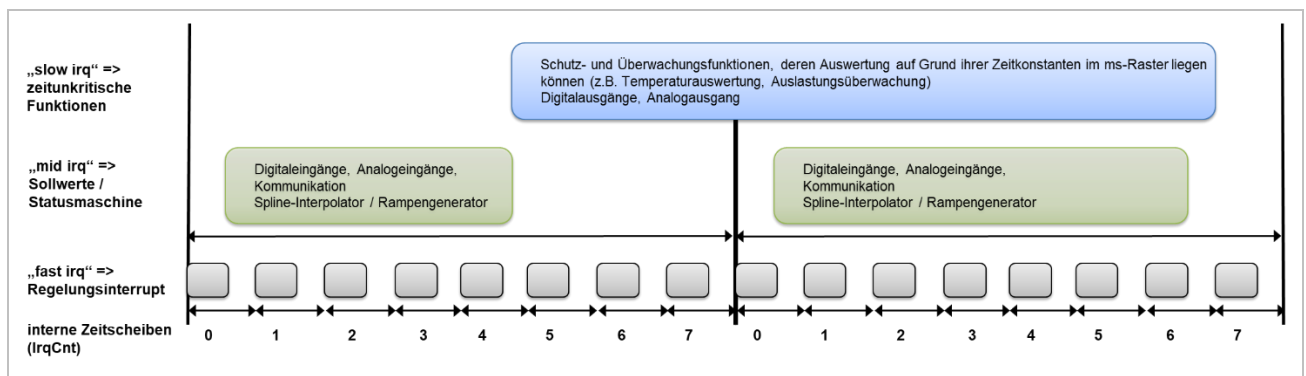
Figure 93: Time allocation
