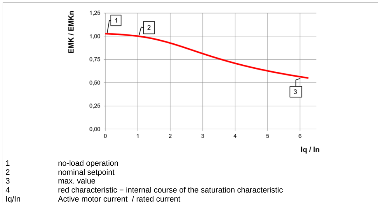
Figure 81: Torque constant depending on the active current
