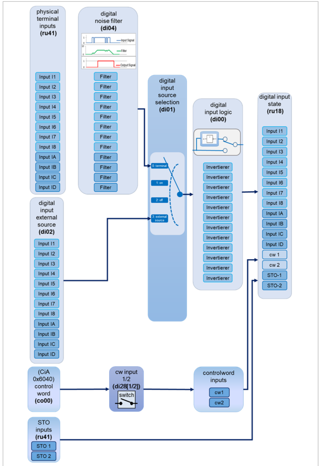
Figure 118: Structure: Evaluation of the digital input status
