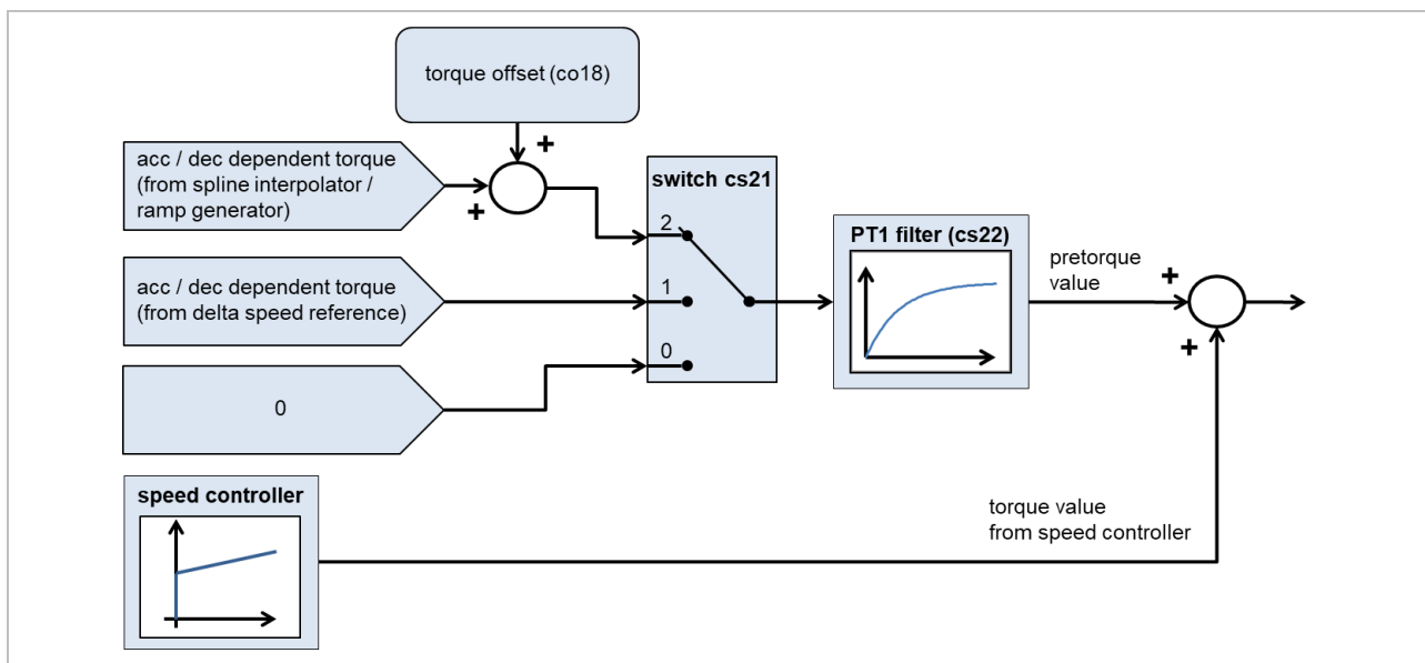
Figure 104: Torque precontrol smoothing
