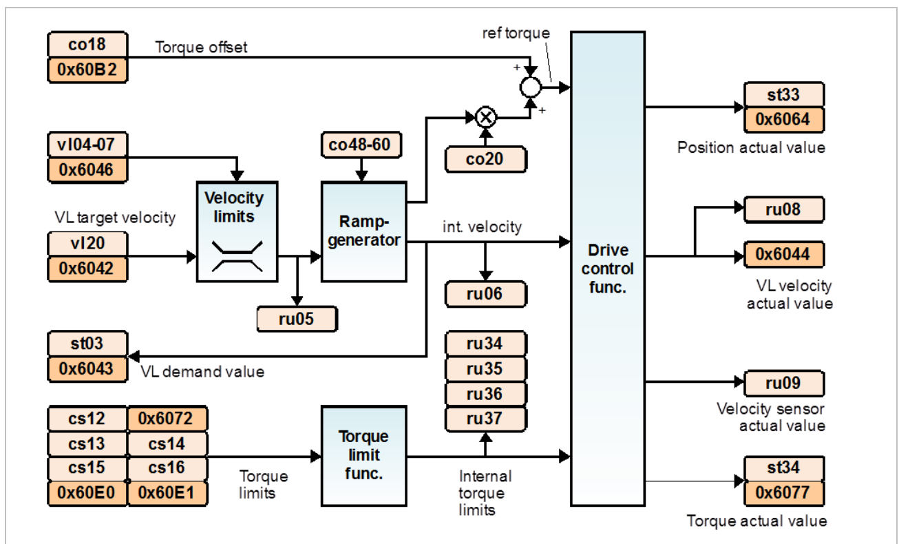
Figure 35: Velocity mode
