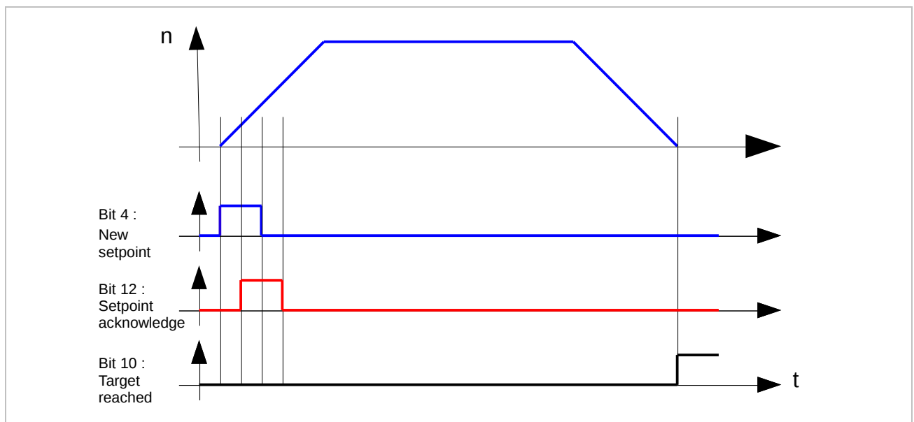
Figure 27: Single positioning
