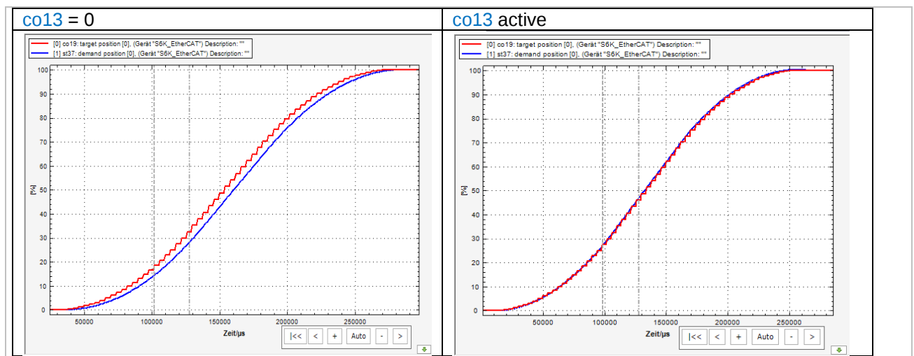
Figure 52: Position precontrol
