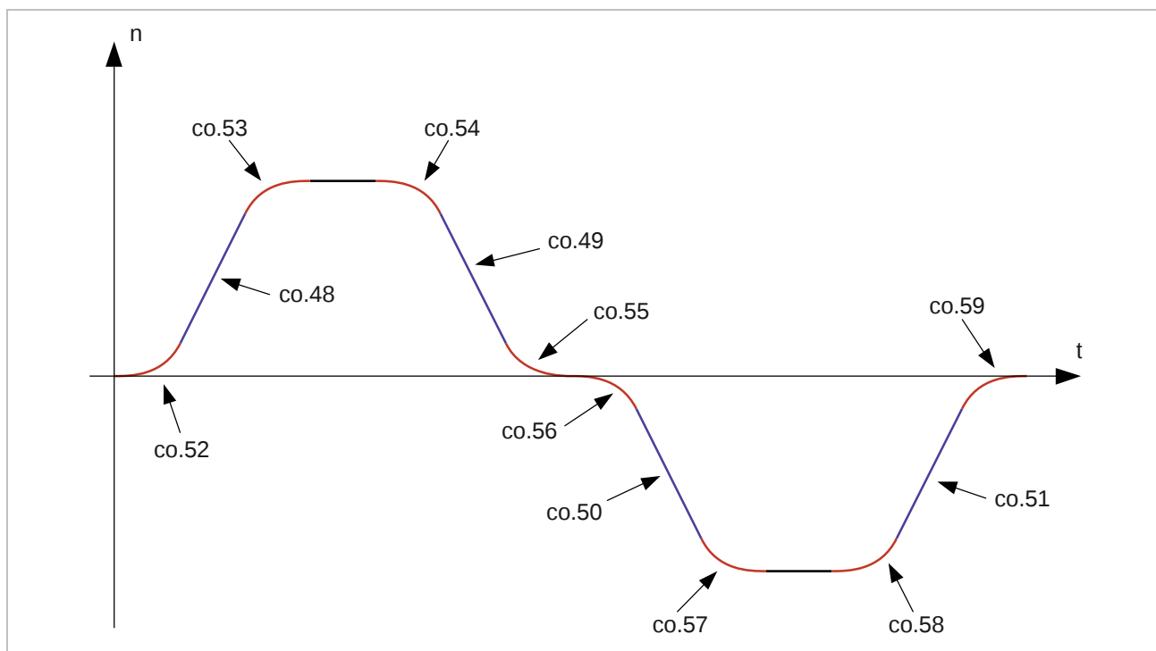
Figure 37: Ramp generator
