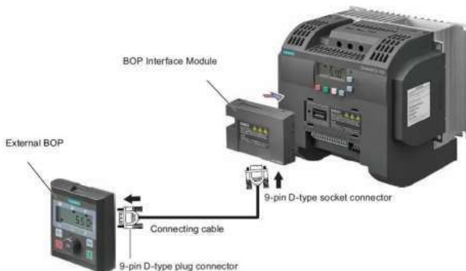
Connecting the external BOP to the BOP interface module
